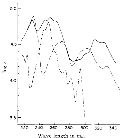
Fig. 1.—Ultraviolet absorption spectra: —, hexahelicene; ---, dibenzo[ c,g ]phenanthrene from E. D. Bergmann and J. S. Szmuszkowicz, THIS JOURNAL , 73 , 5153 (1951); - · - · -, phenanthrene, from R. A. Friedel and M. Orchin, "Ultraviolet Spectra of Aromatic Compounds," John Wiley and Sons, Inc., New York, N. Y., 1951, structure 341.
